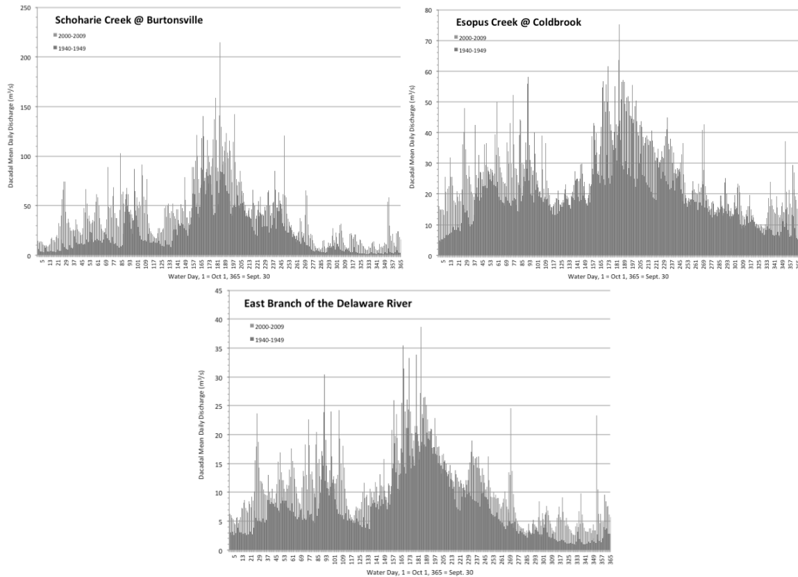
Figure 2: Mean daily discharge for each day during the decade (2000-2009 or 1940-1949) for streams on the north, south and southwest edges of the Catskills.
