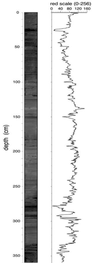
The sediment core from YLN and the red color intensity scale highlighting fld layers. The flood layer from Hurricane Irene is visible at the very top of the core
