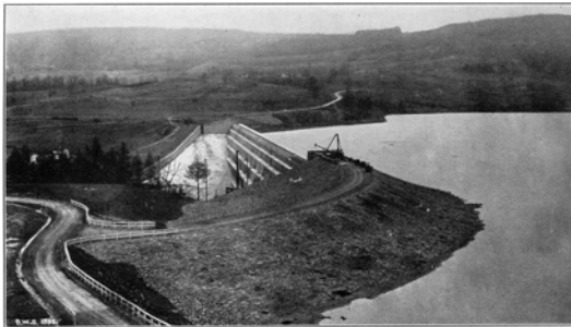
The Gilboa Dam –Construction nearly complete.
