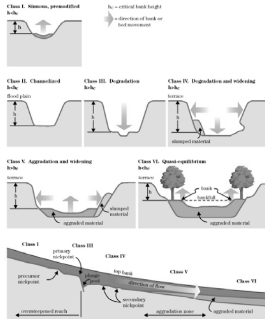
Figure 1: Simon Channel Evolution Model (1989), from USDA/NRCS Technical Note 4 “Understanding Fluvial Systems: Wetlands, Streams, and Flood Plains (2010)”
